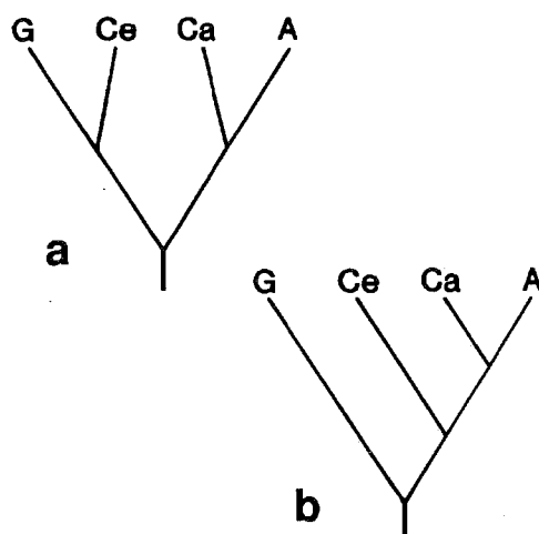
Figure 1. The two most likely alternative phylogenies of Gymnostoma (G), Ceuthostoma (Ce), Casuarina (Ca), and Allocasuarina (A). All internodes would represent at least one synapomorphy.
